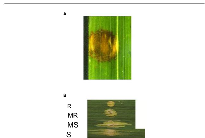
Figure 2: Reactions in leaves of rice accessions at 15 days after infiltration with MAI3, MAI10 and BLS256. Phenotypes were photographed on a light box. (A) Hypersensitive reaction (HR), visible as browning in response to MAI3 and MAI10 on FKR14 leaves; (B) Scale used to assess disease level: Resistant (R), 0<LL ≤ 1mm; Moderately Resistant (MR), 1<LL ≤ 10 mm; Moderately susceptible (MS), 10<LL ≤ 30 mm; Susceptible (S), LL>30 mm.
