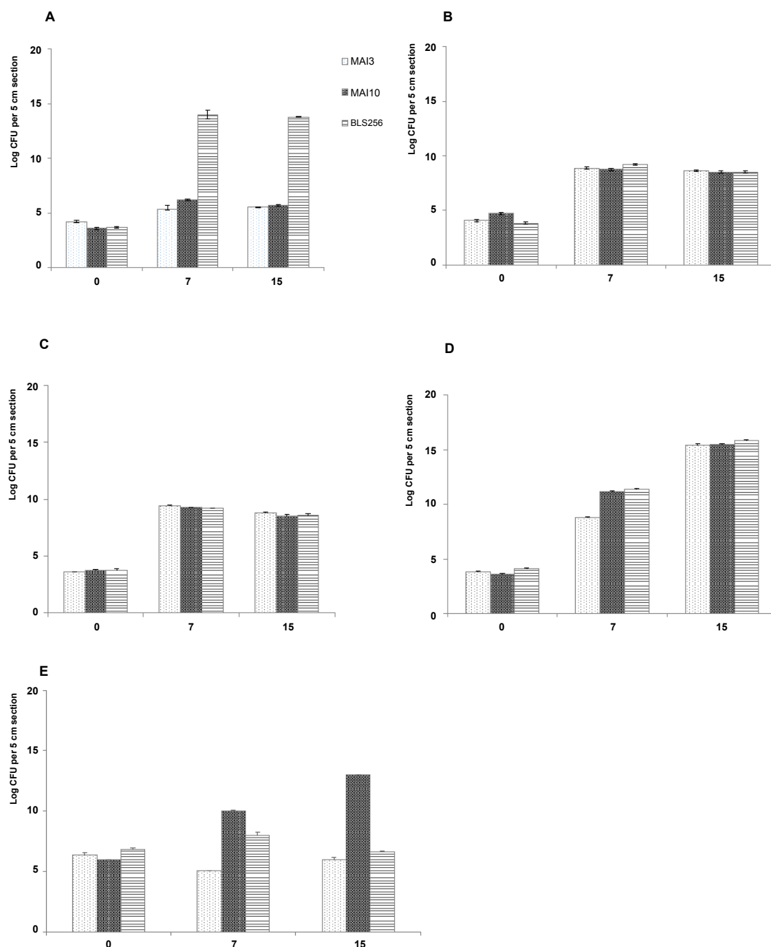
Figure 3: Bacterial growth in 3-week-old leaves of FKR14 (A), TOG5672 (B), TOG6767 (C), TN1 (D) rice accessions and transgenic line Kitaake-Rxo1 (E). Bacterial population was measured in a 5 cm leaf segment around the infiltration point at 0, 7 and 15 days after inoculation with Xoc strains MAI3, MAI10 and BLS256. The experiment was repeated three times. Error bars represent standard error.
