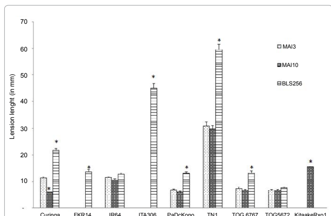
Figure 1: Lengths of lesions caused by X. oryzae pv. oryzicola strains BLS256, MAI10 and MAI3 on six rice accessions of O. sativa sp. Indica , two accessions of O. glaberrima (TOG6767, TOG5672) and transgenic indica line Kitaake-Rxo1. Lesions were measured 15 days after infiltration. An asterisk denotes a significant difference between BLS256 and African Xoc (*, P<0.05). The experiment was repeated three times with similar results.
